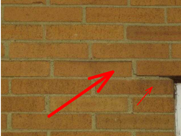
Stress Cracks With Displacement
